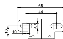
L型支架安装孔 L-Bracket Mounting Hole
